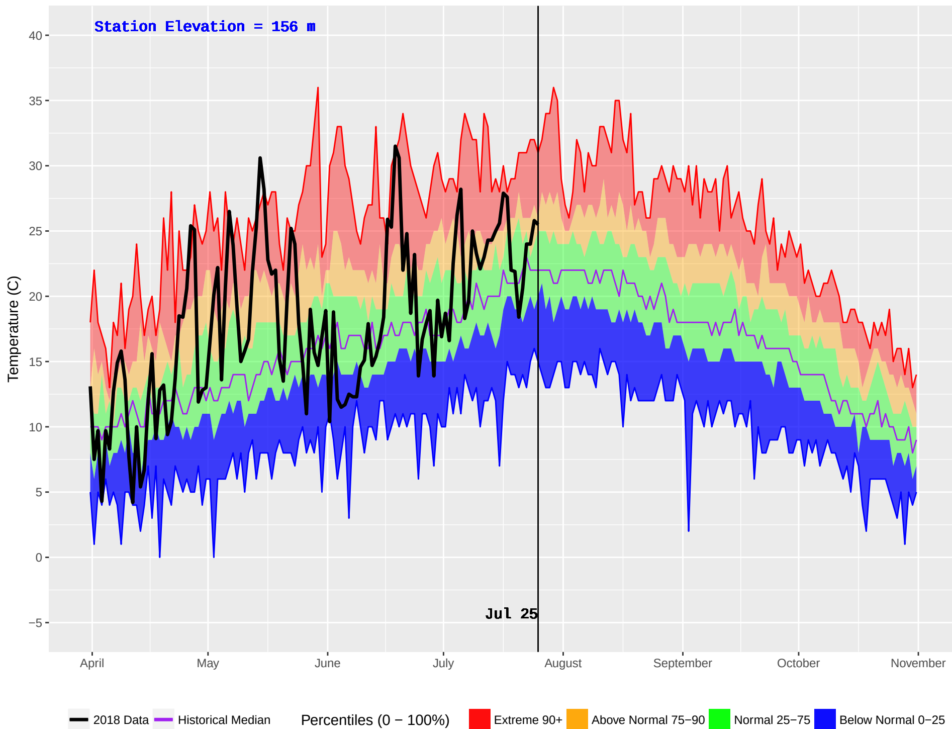
WOSS CAMP (21) : Historical (1970–2016) and Current (2018) Noon Temperature
