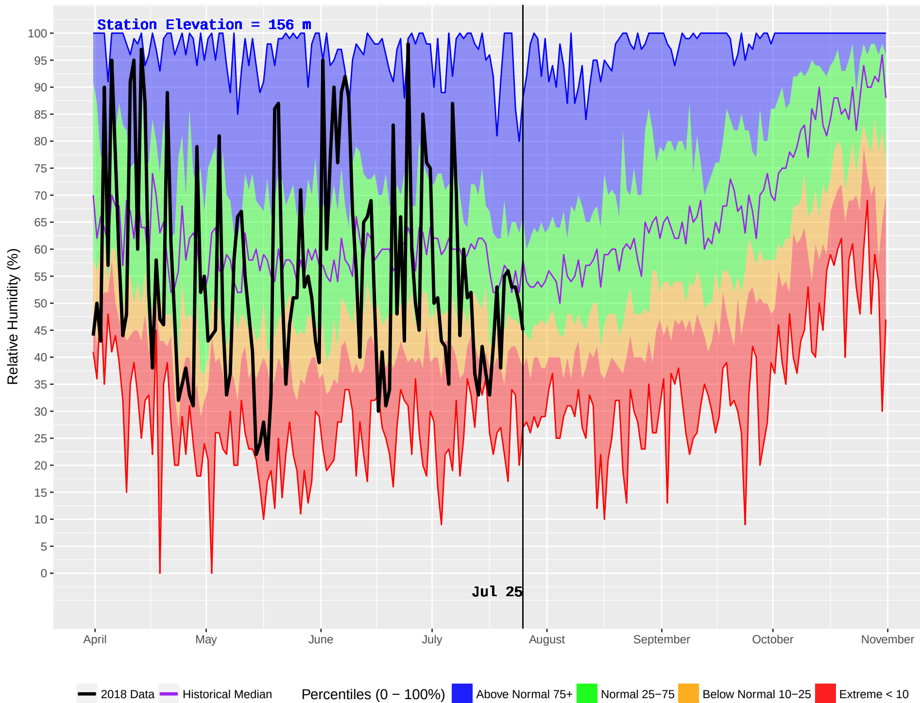
WOSS CAMP (21) : Historical (1970–2016) and Current (2018) Noon Relative Humidity
