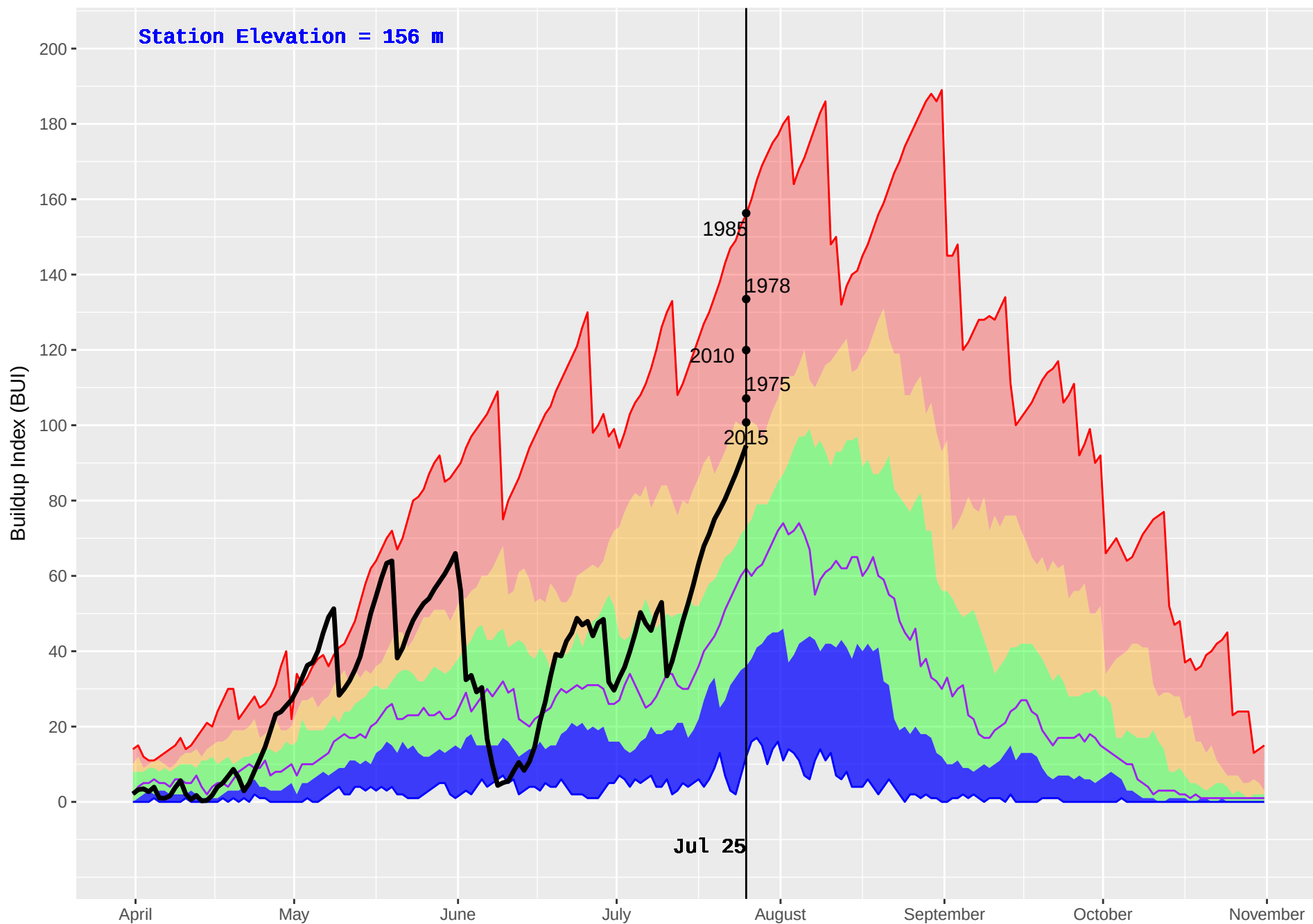
WOSS CAMP (21) : Historical (1970–2016) and Current (2018) Noon Buildup Index (BUI)
