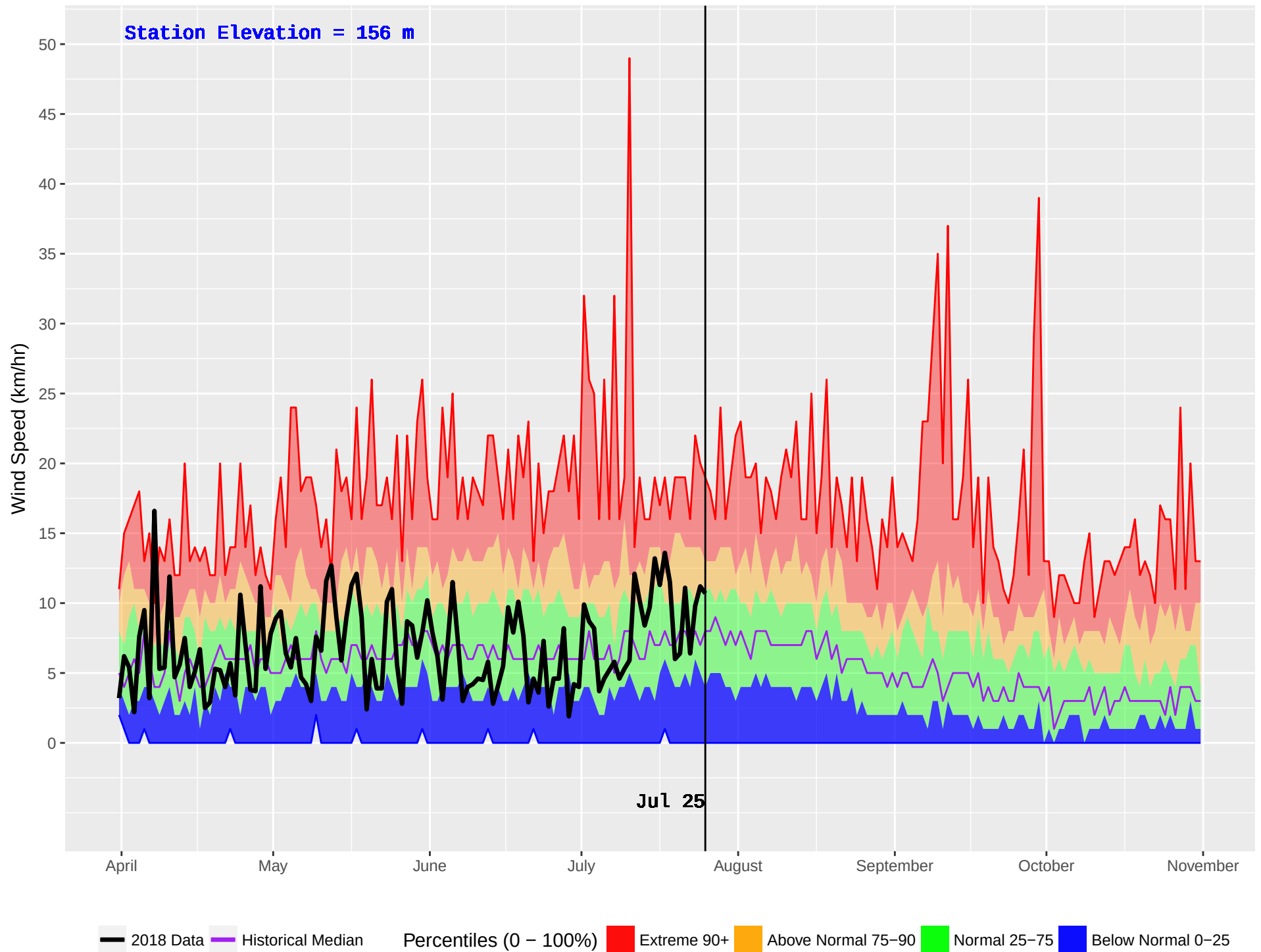
WOSS CAMP (21) : Historical (1970–2016) and Current (2018) Noon Wind Speed
