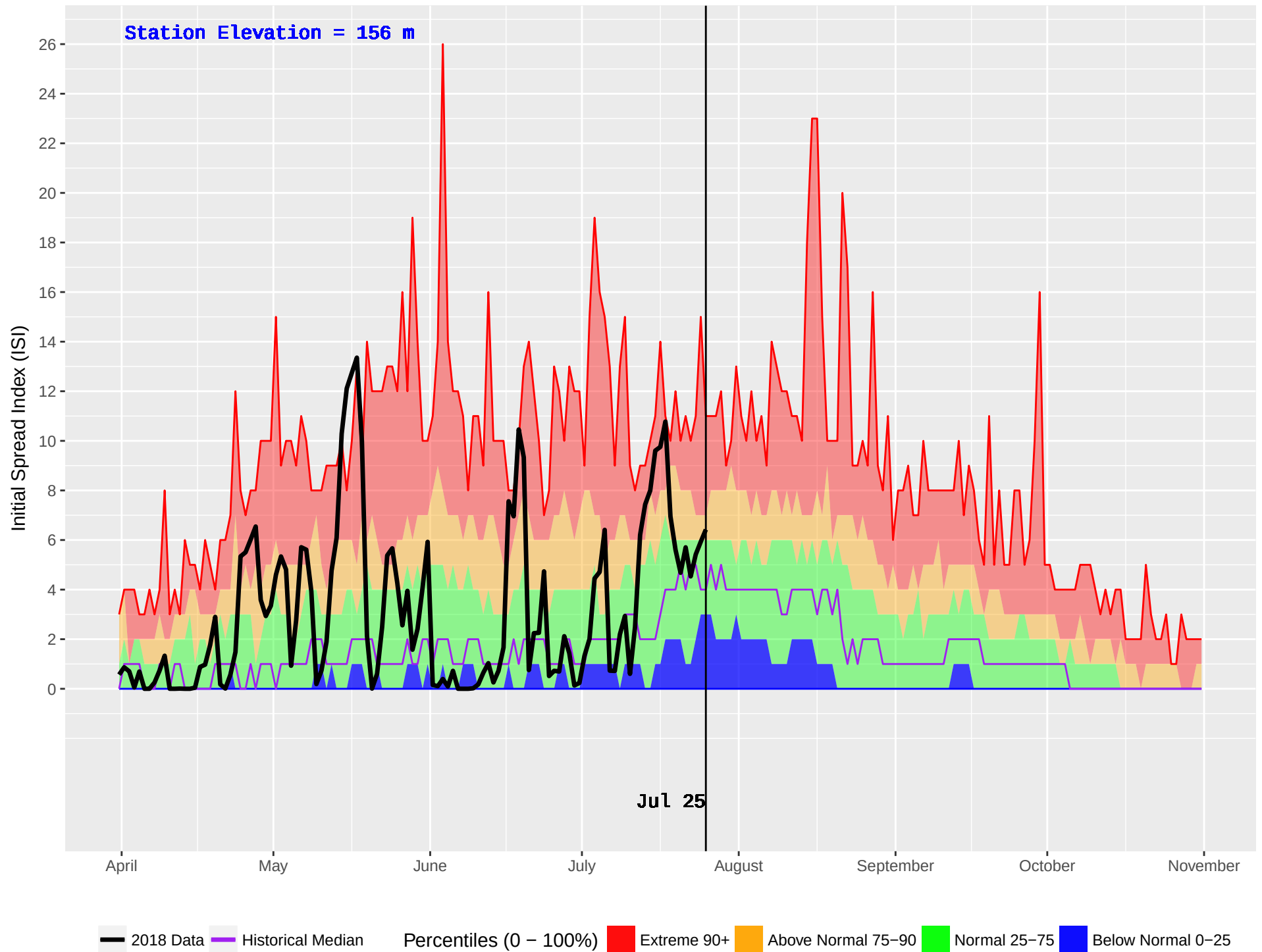
WOSS CAMP (21) : Historical (1970–2016) and Current (2018) Noon Initial Spread Index (ISI)
