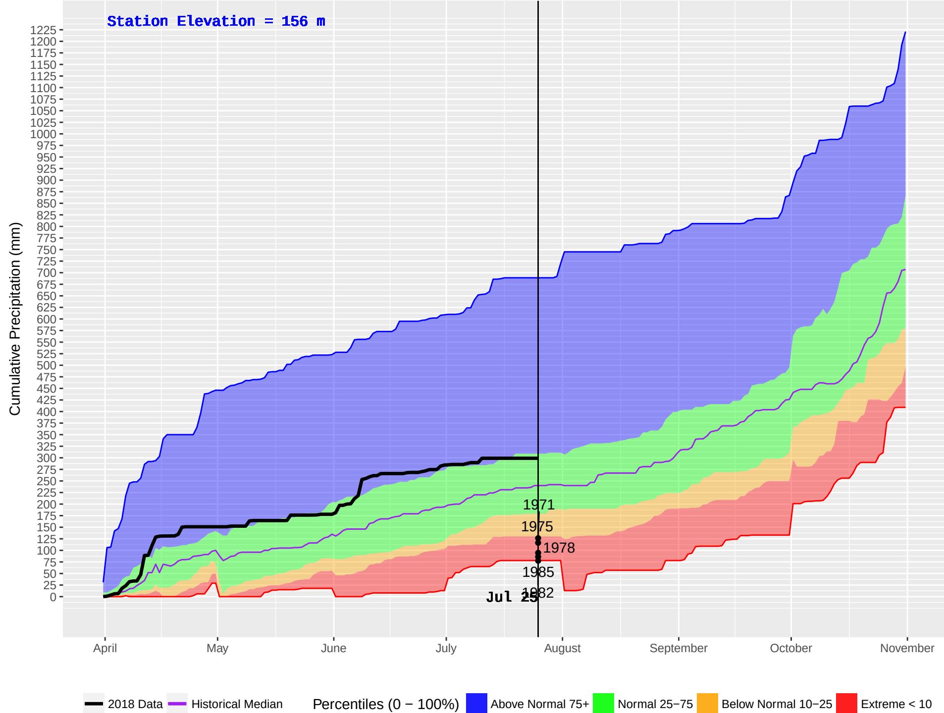
WOSS CAMP (21) : Historical (1970–2016) and Current (2018) Noon Cumulative Precipitation
